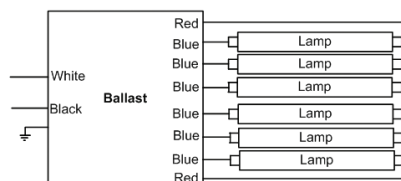
(3) 6-lamp wiring
